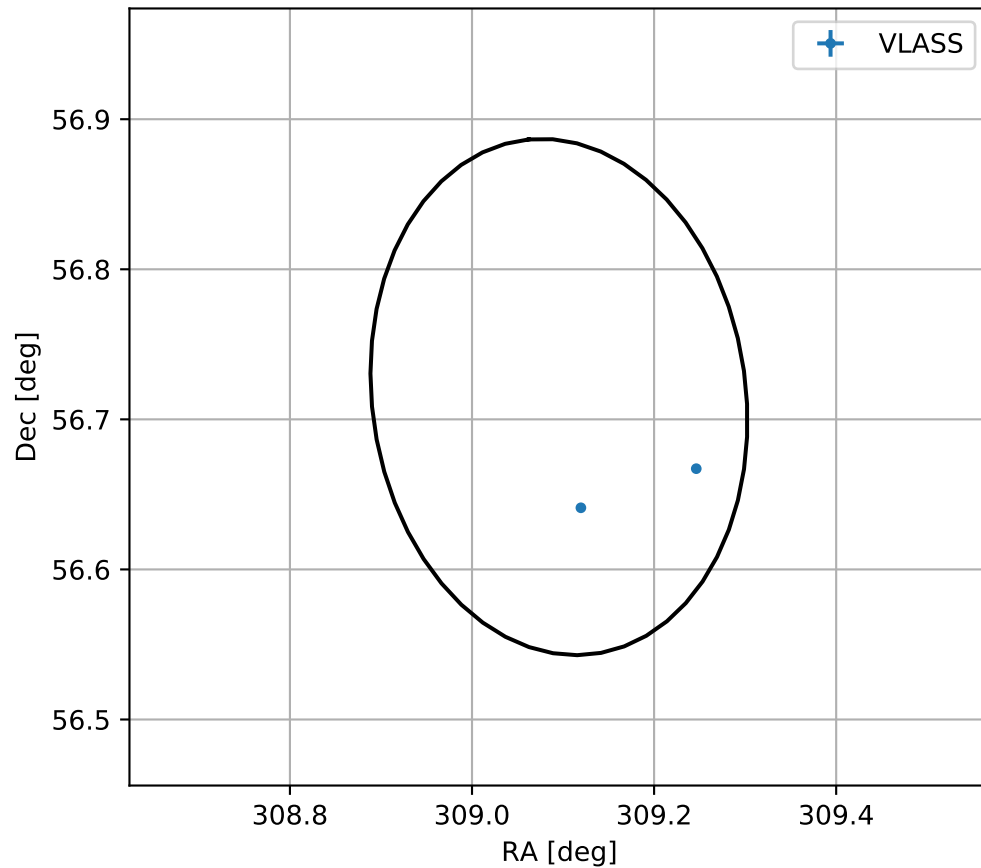
4FGL J2036.3+5642c
