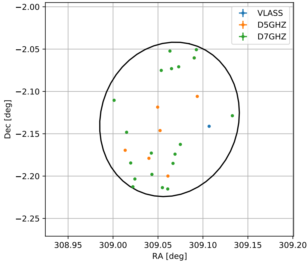
4FGL J2036.2-0207
