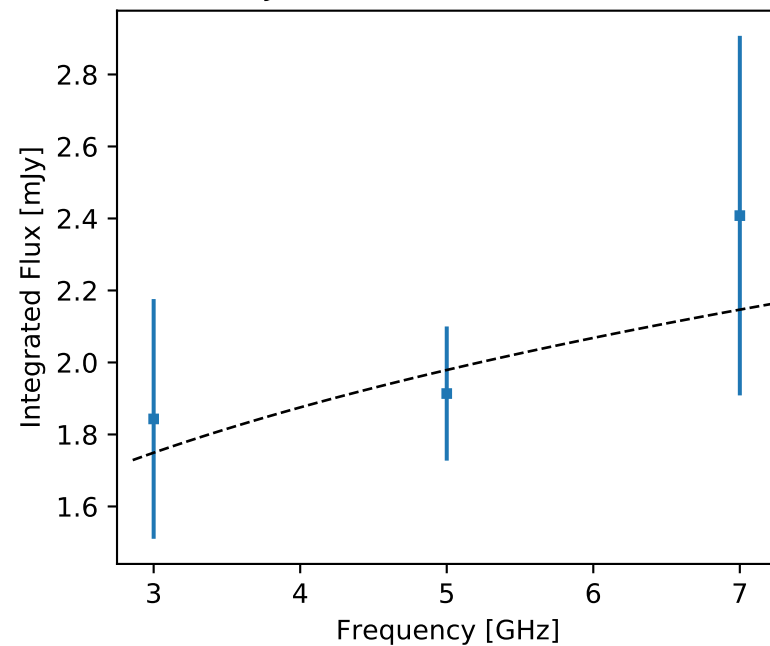
F357 J203505.79+363146.5 (unr)
