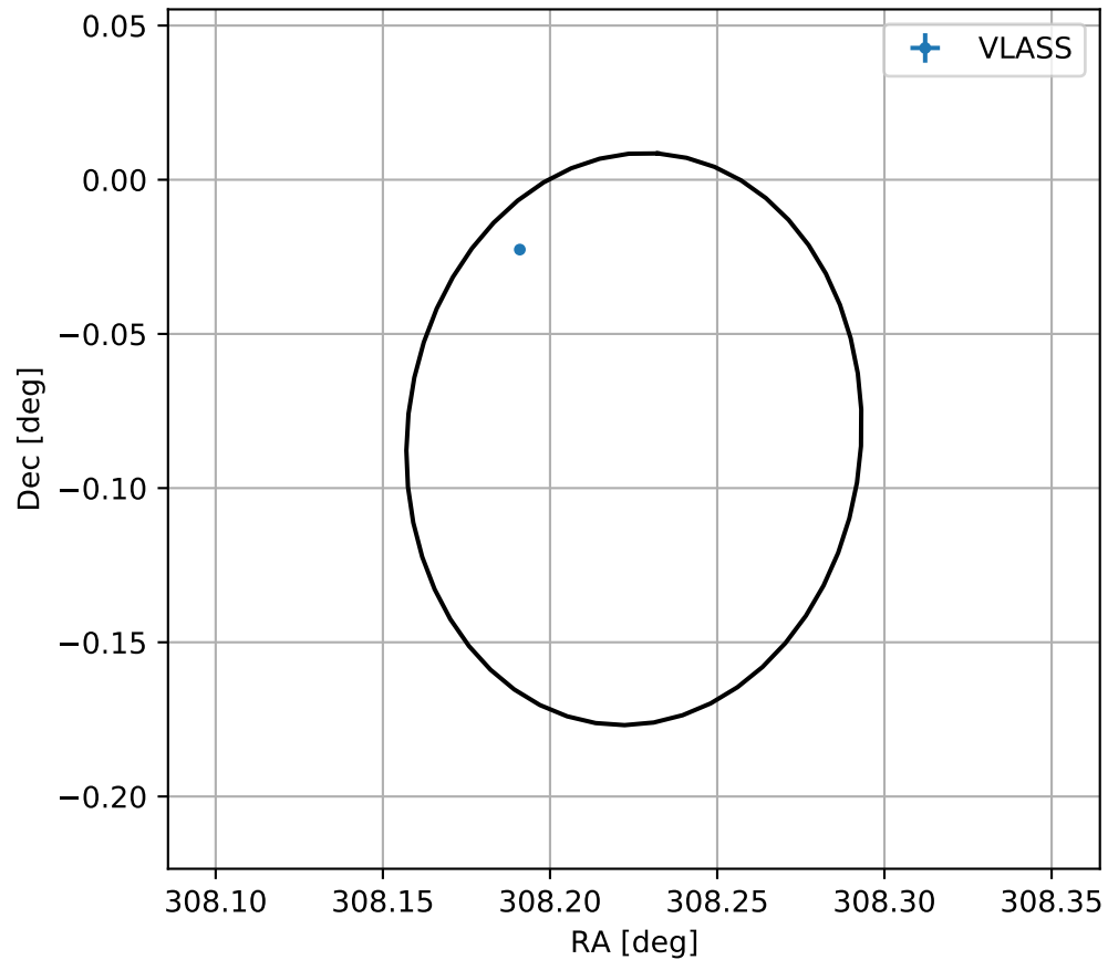
4FGL J2032.9-0005
