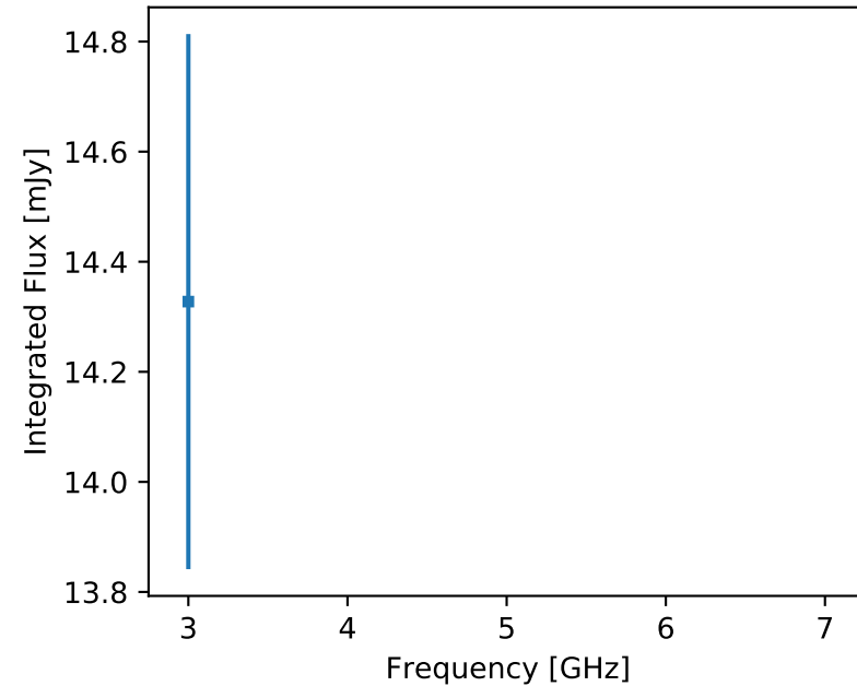
F357 J203245.83-000121.5 (unr)
