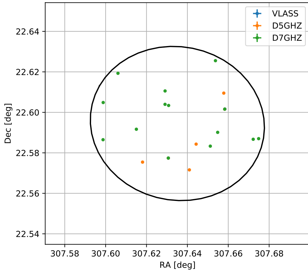
4FGL J2030.5+2235
