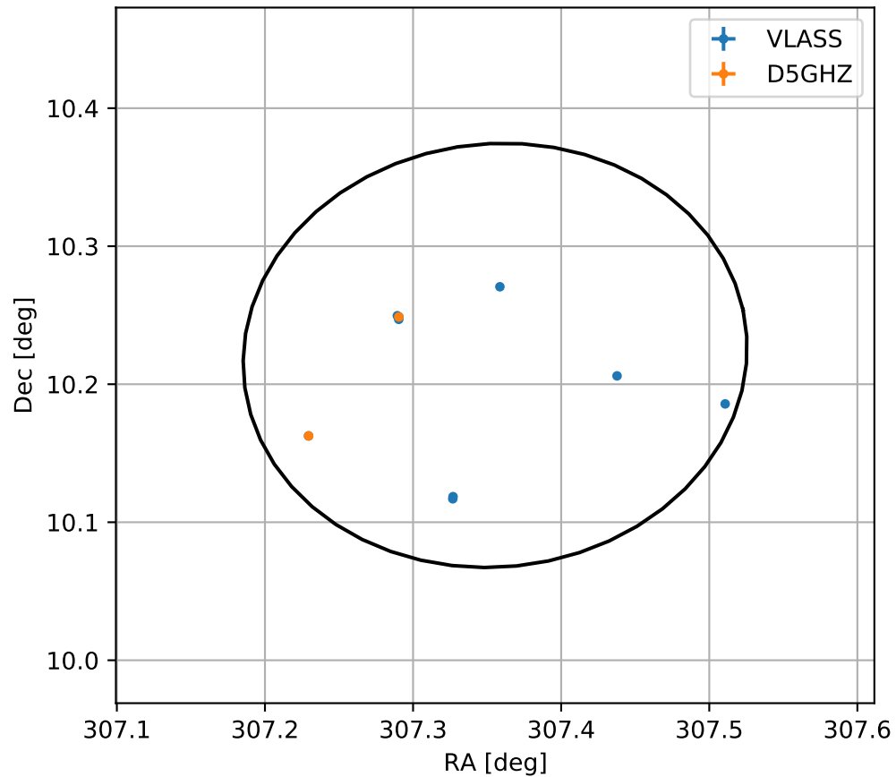
4FGL J2029.4+1013
