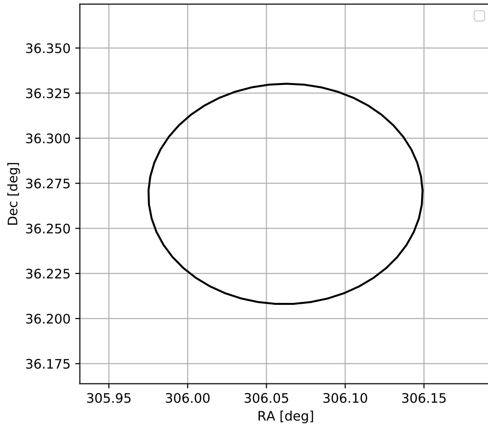
4FGL J2024.2+3616
