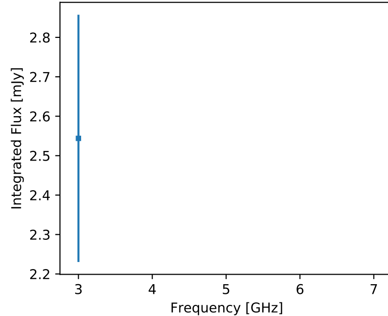
F357 J202306.01-194732.5 (unr)
