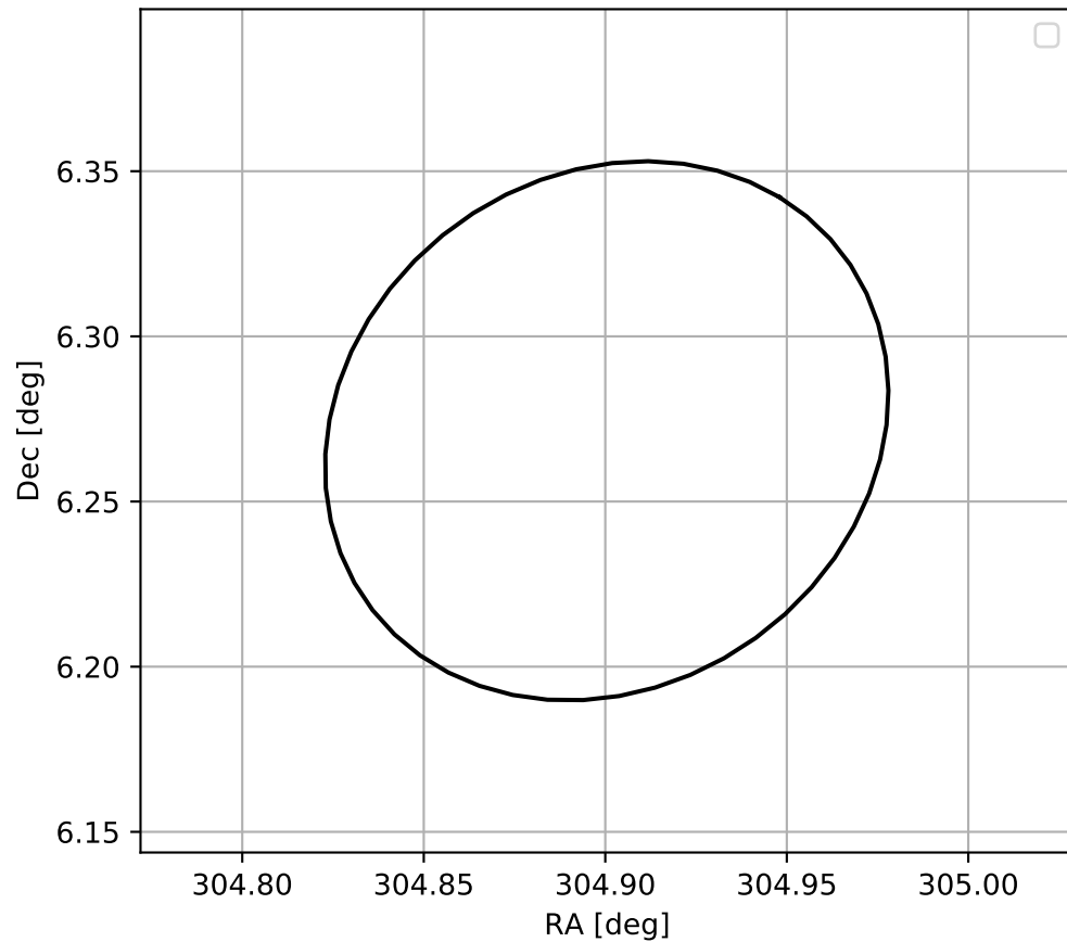
4FGL J2019.6+0616
