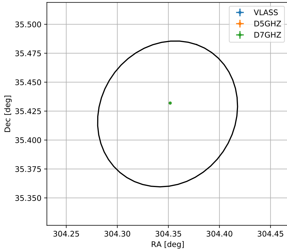
4FGL J2017.3+3525
