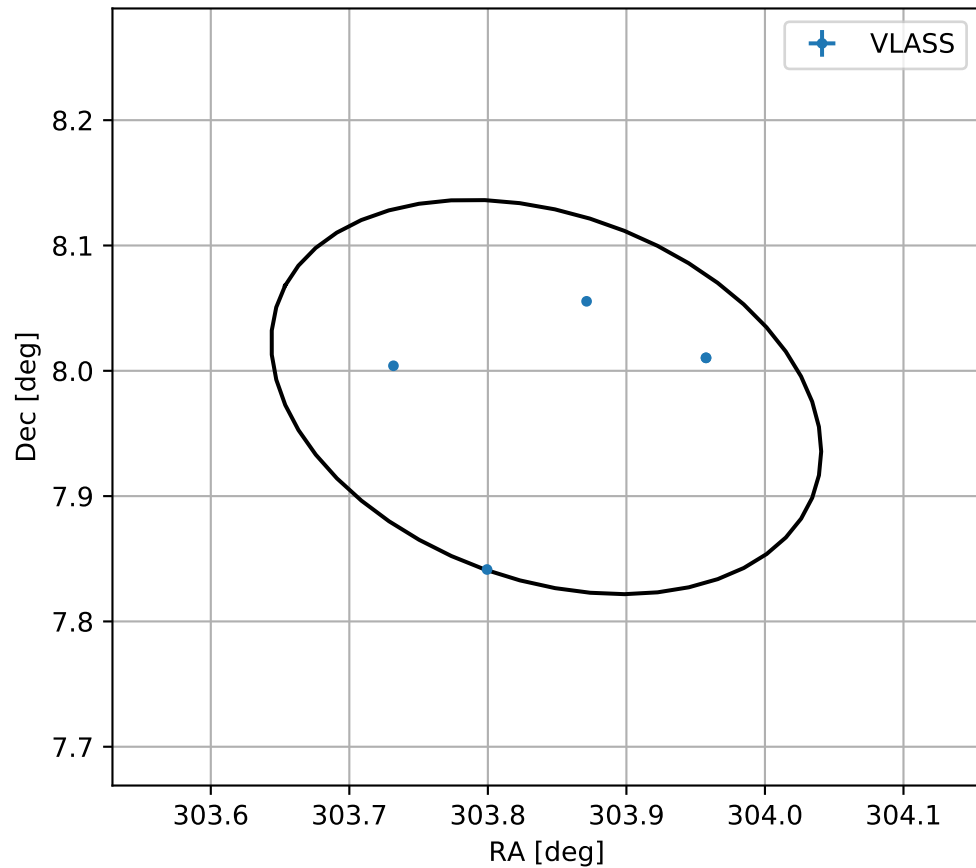
4FGL J2015.3+0758
