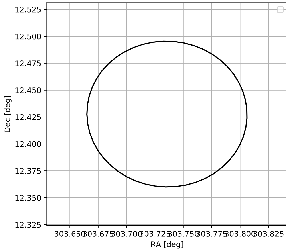
4FGL J2014.9+1225
