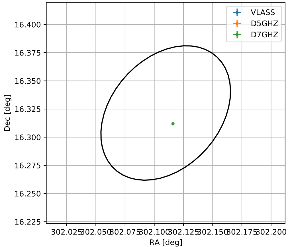
4FGL J2008.4+1619
