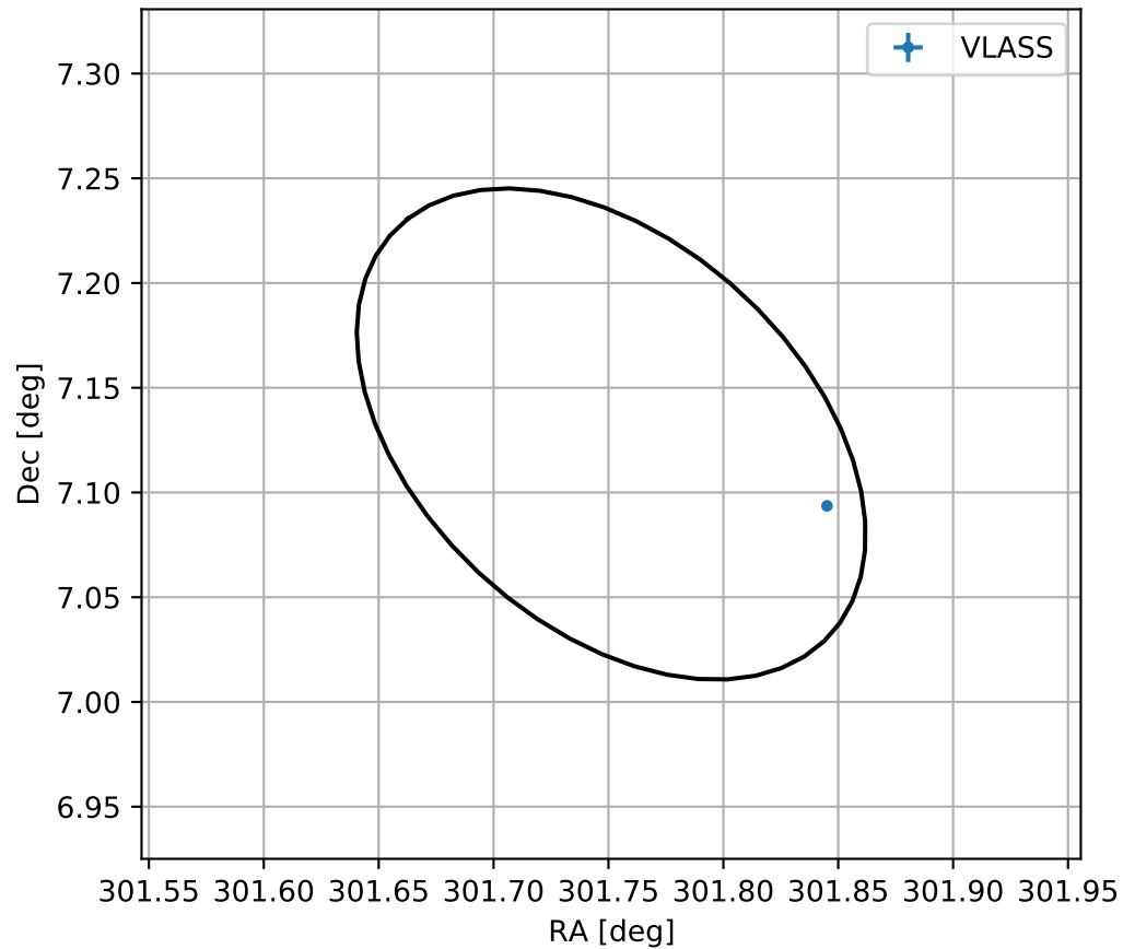
4FGL J2007.0+0707
