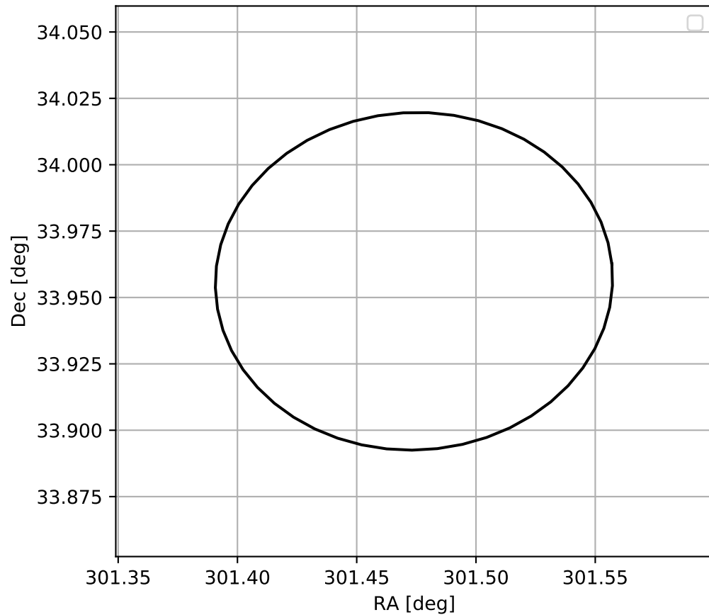
4FGL J2005.8+3357
