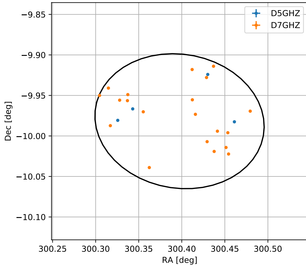
4FGL J2001.5-0958
