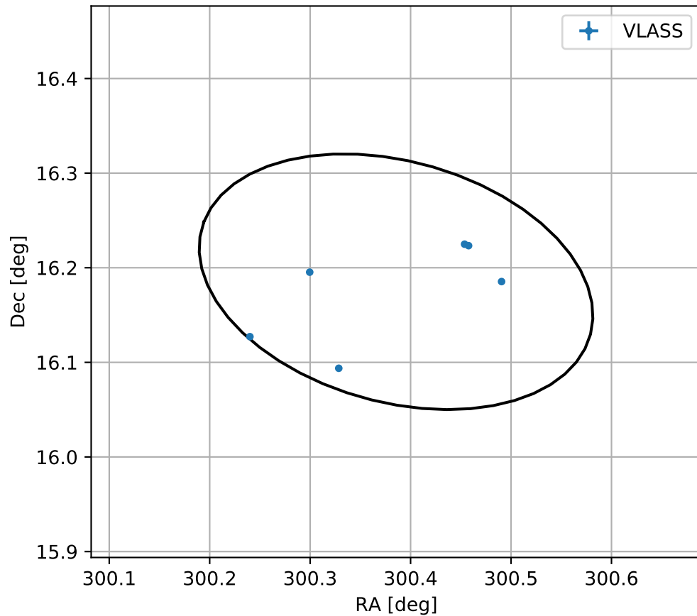
4FGL J2001.5+1611
