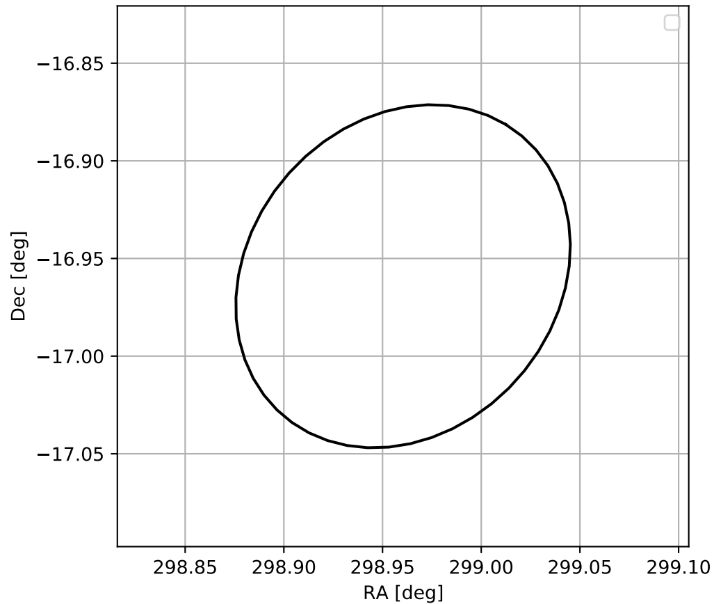
4FGL J1955.8-1657
