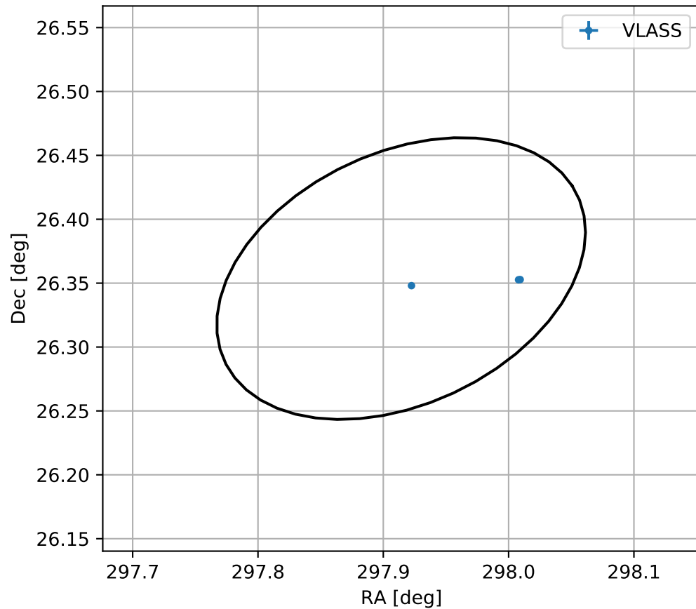
4FGL J1951.6+2621
