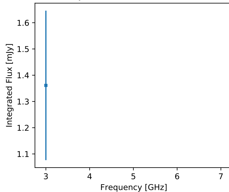
F357 J195202.21+262110.0 (res)
