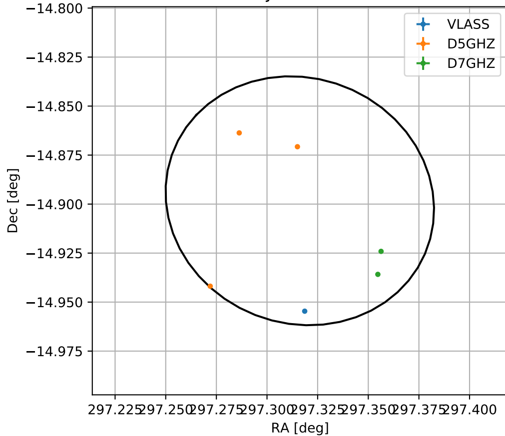
4FGL J1949.2-1453
