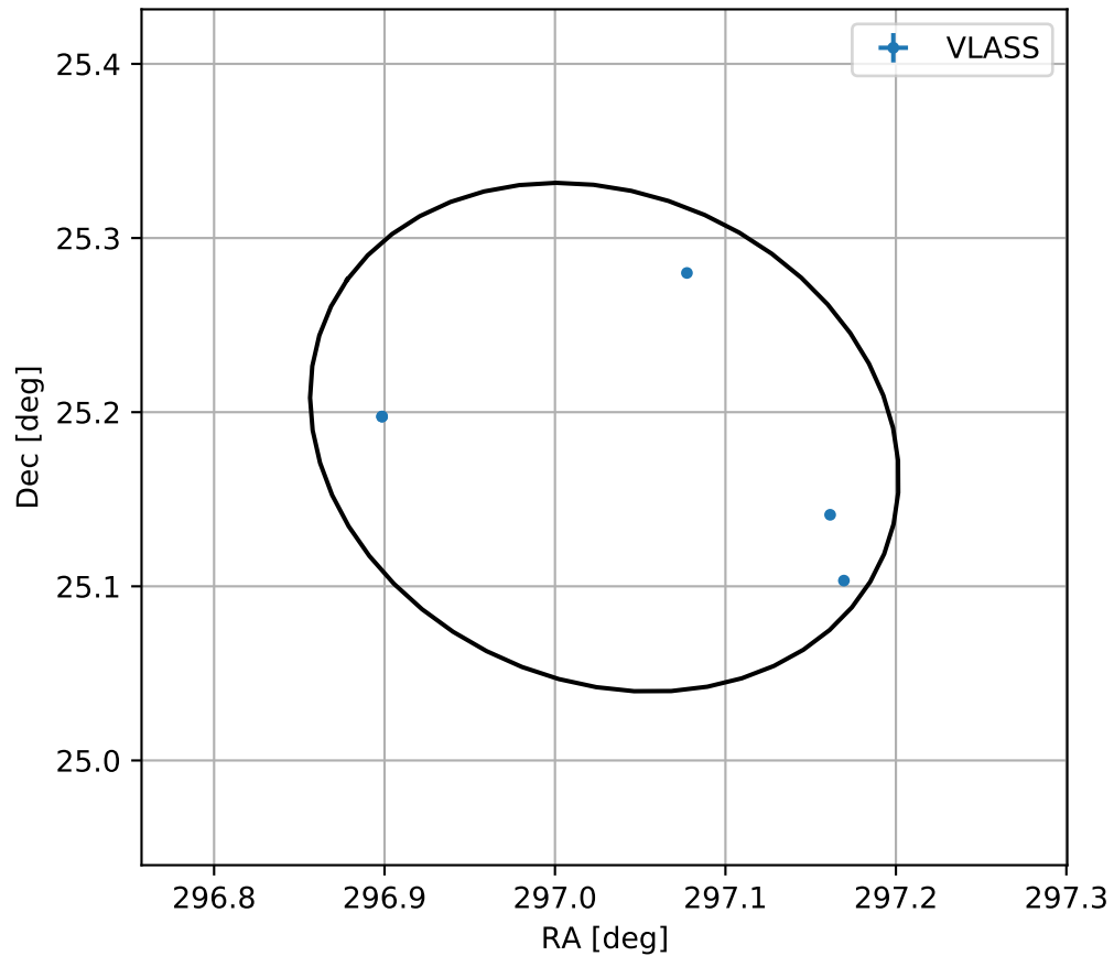
4FGL J1948.1+2511
