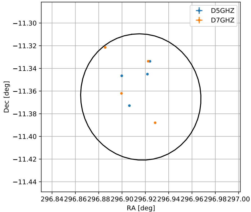
4FGL J1947.6-1121
