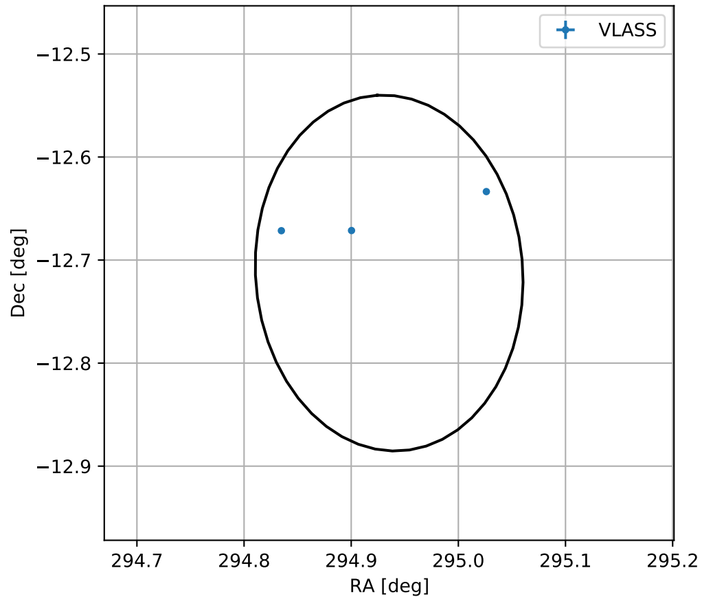
4FGL J1939.7-1242
