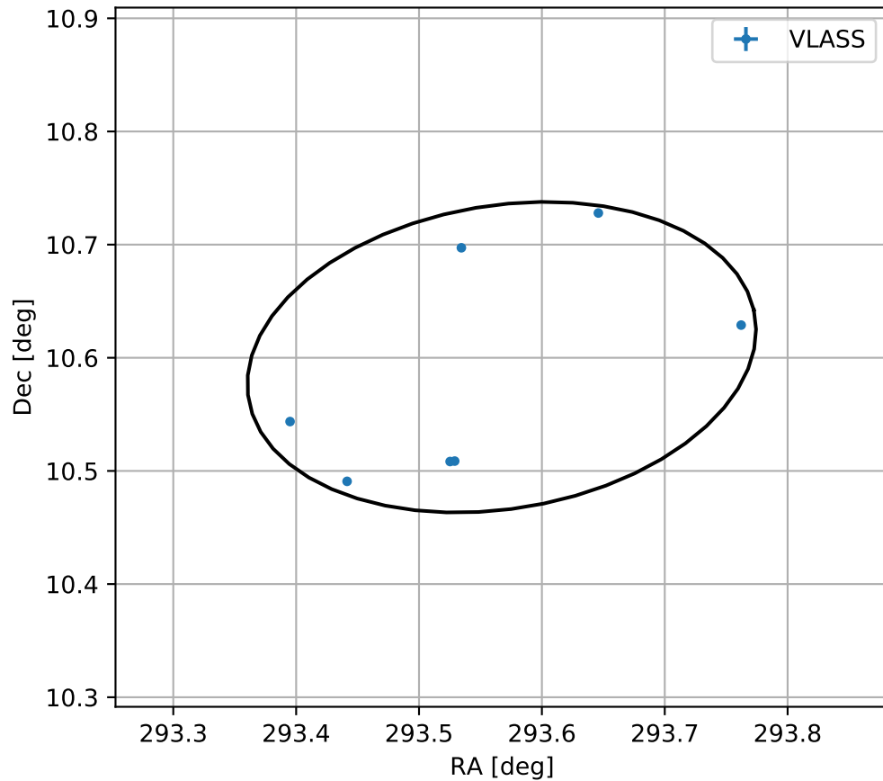
4FGL J1934.2+1036
