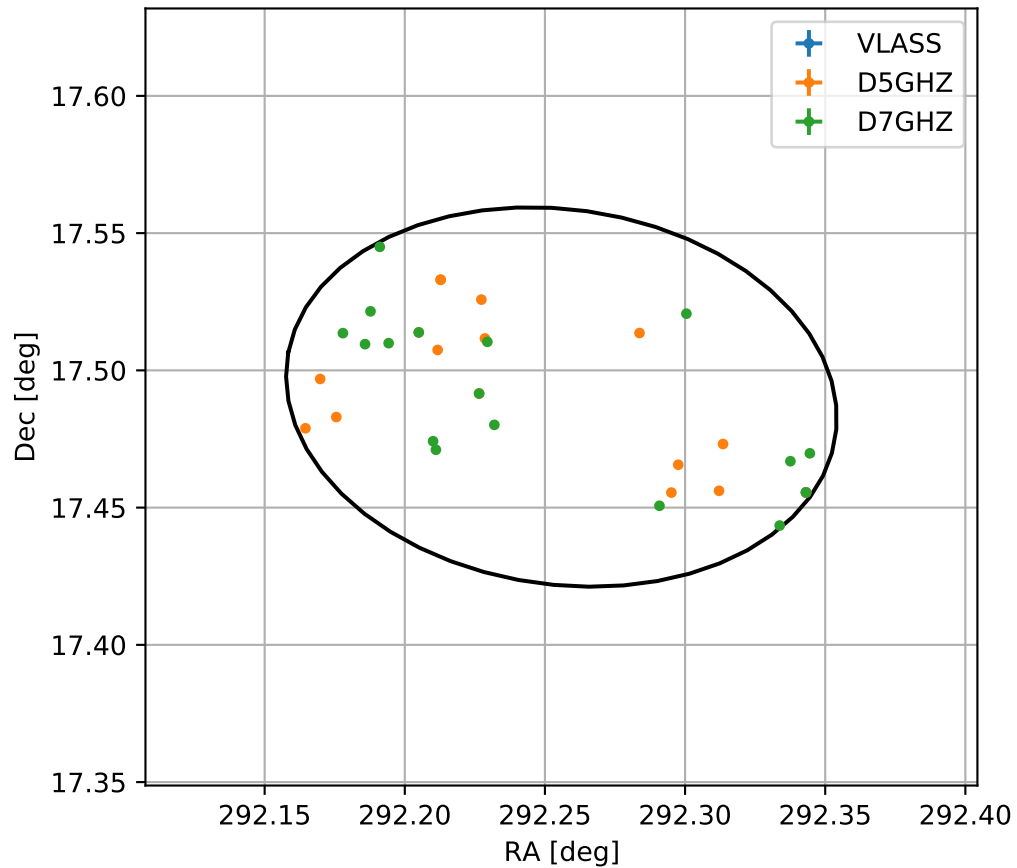
4FGL J1929.0+1729
