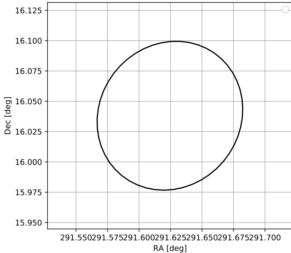
4FGL J1926.4+1602
