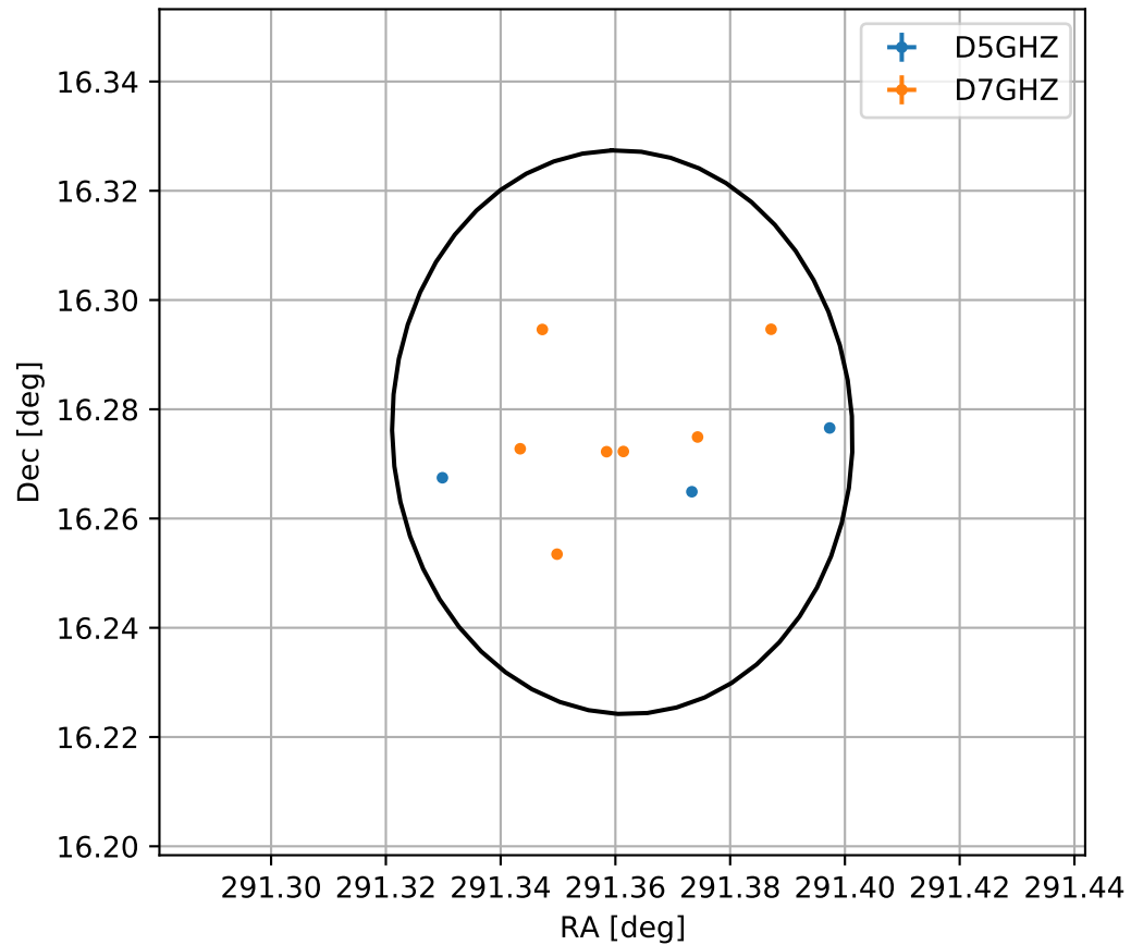
4FGL J1925.4+1616
