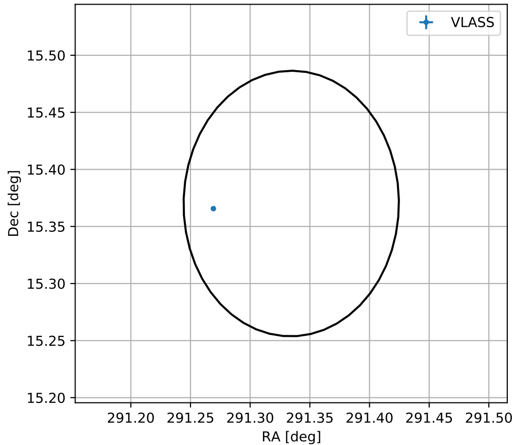
4FGL J1925.3+1522c
