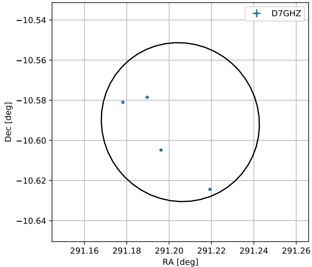
4FGL J1924.8-1035
