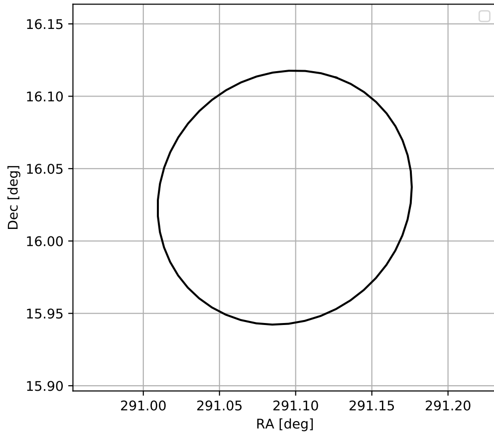
4FGL J1924.3+1601c
