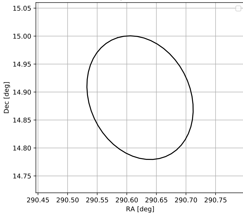
4FGL J1922.4+1453c
