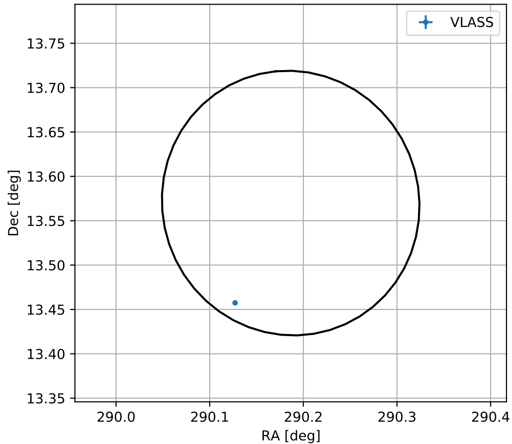
4FGL J1920.7+1334
