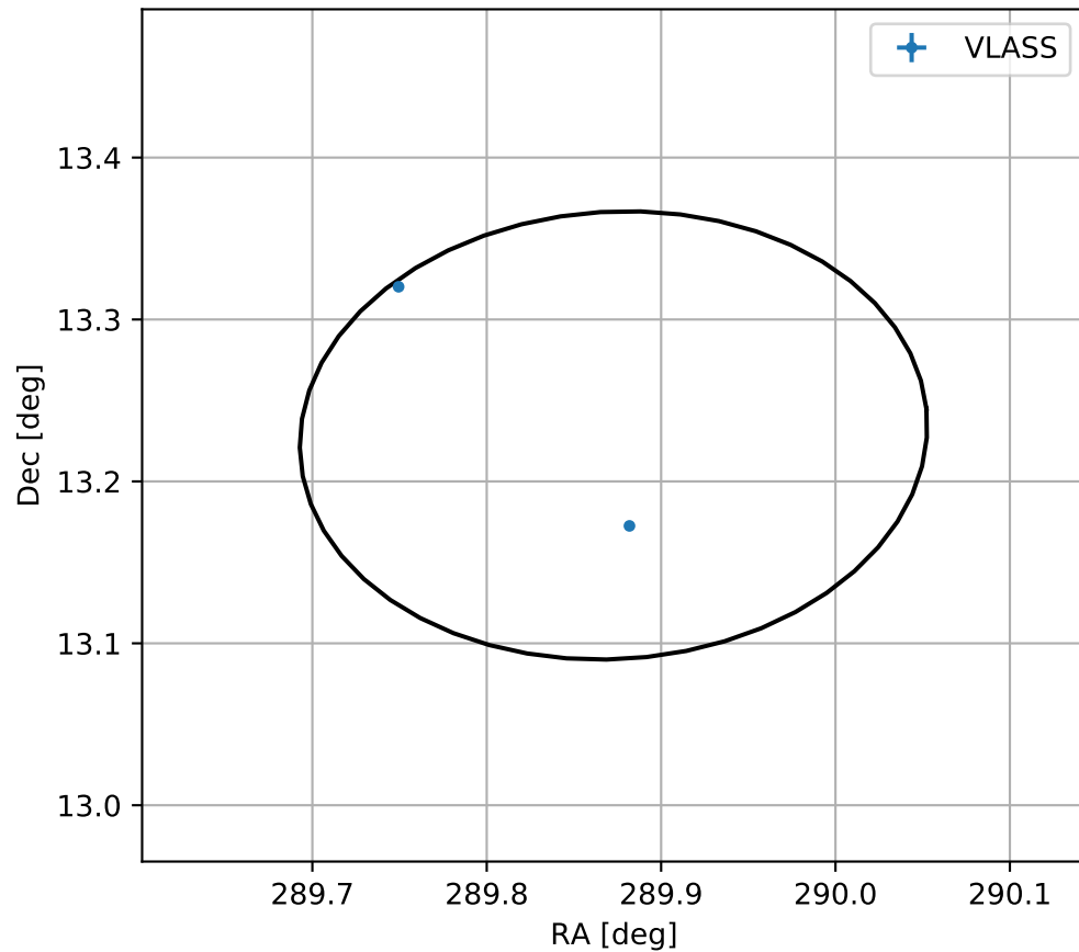
4FGL J1919.4+1313
