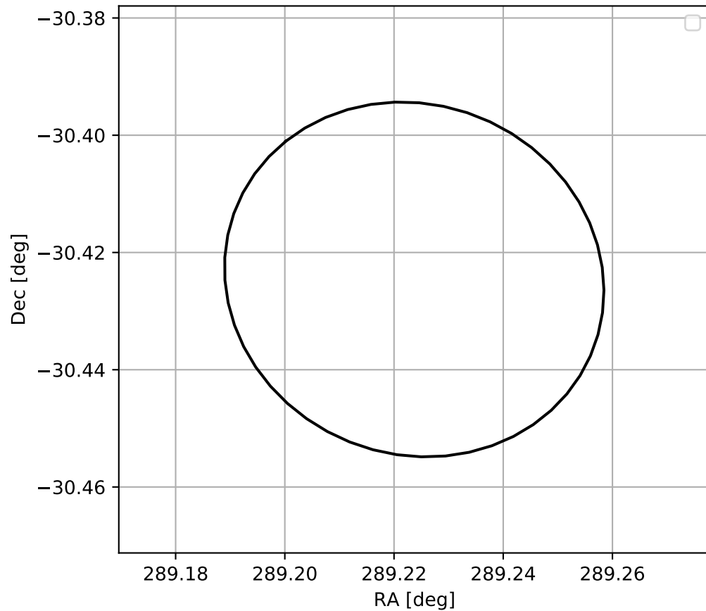
4FGL J1916.8-3025
