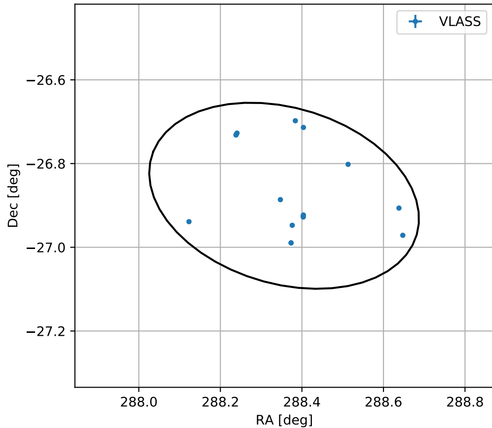
4FGL J1913.4-2652
