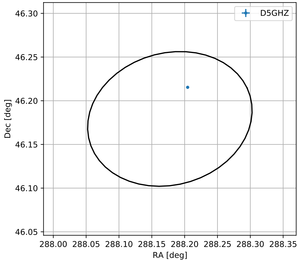
4FGL J1912.7+4610
