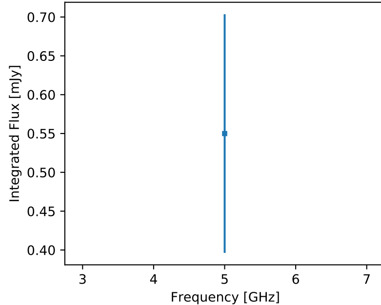
F357 J191249.09+461255.3 (unr)
