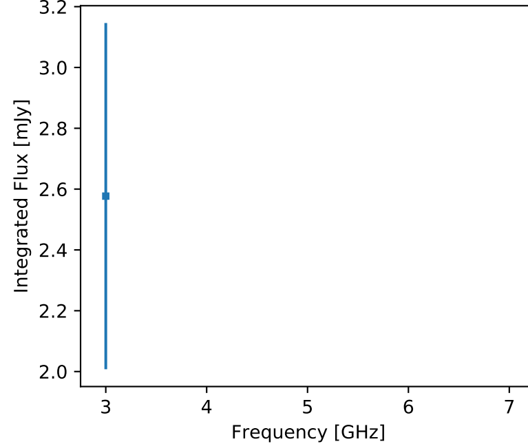
F357 J191230.10+131206.2 (unr)
