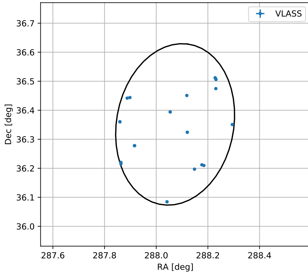
4FGL J1912.2+3621
