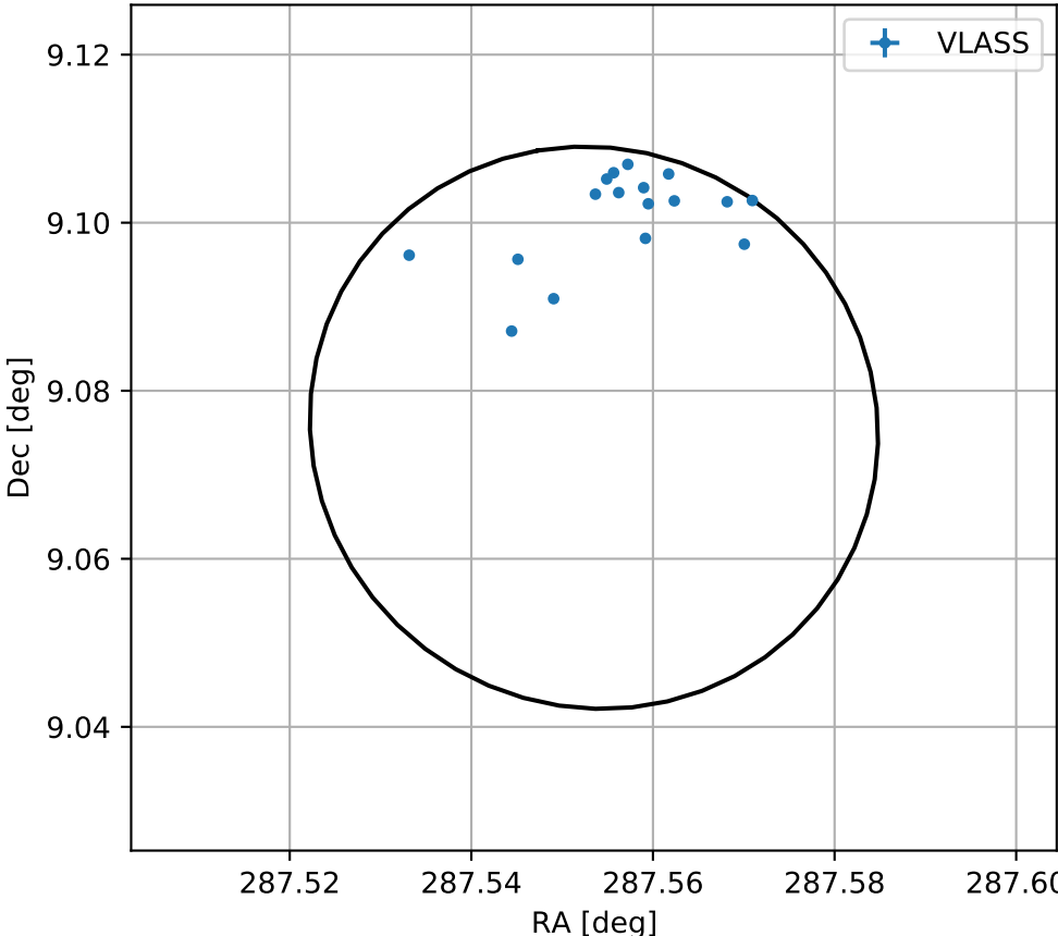
4FGL J1910.2+0904c
