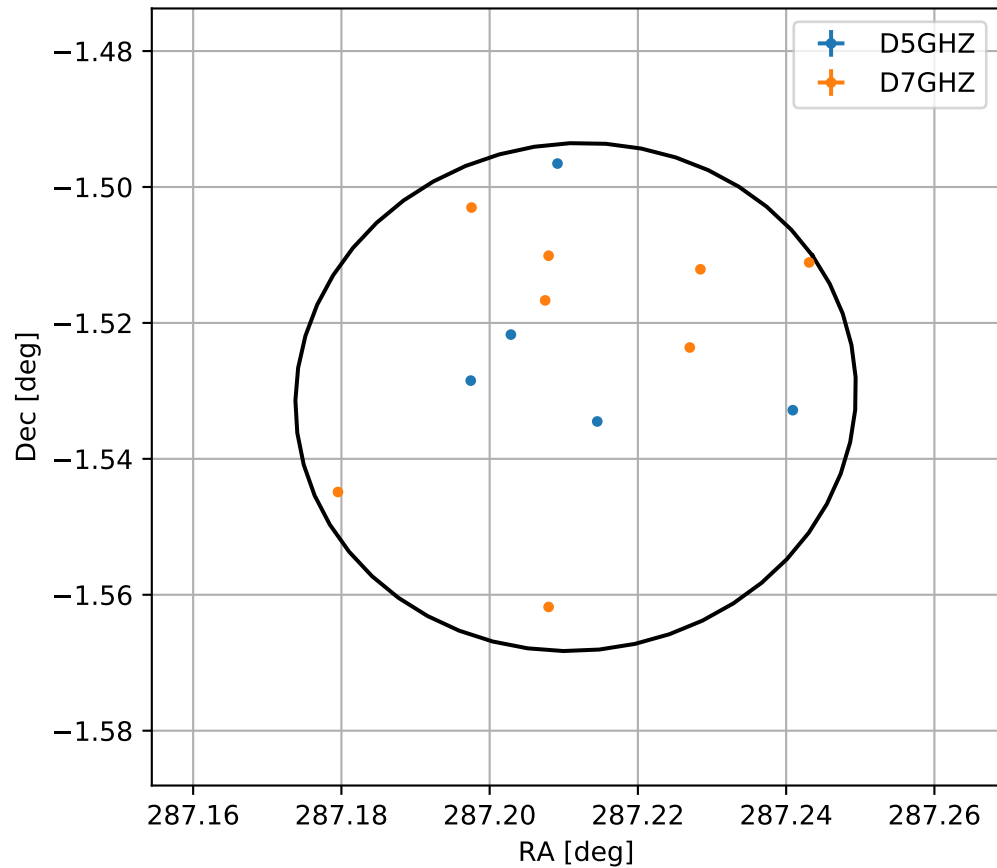
4FGL J1908.8-0131
