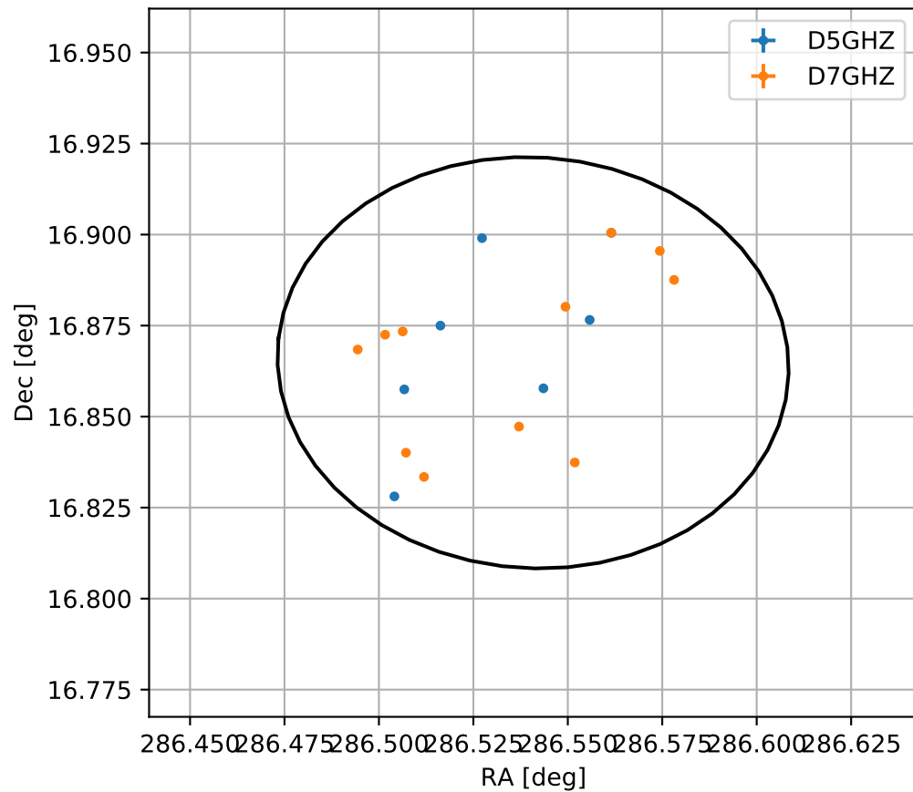
4FGL J1906.1+1651
