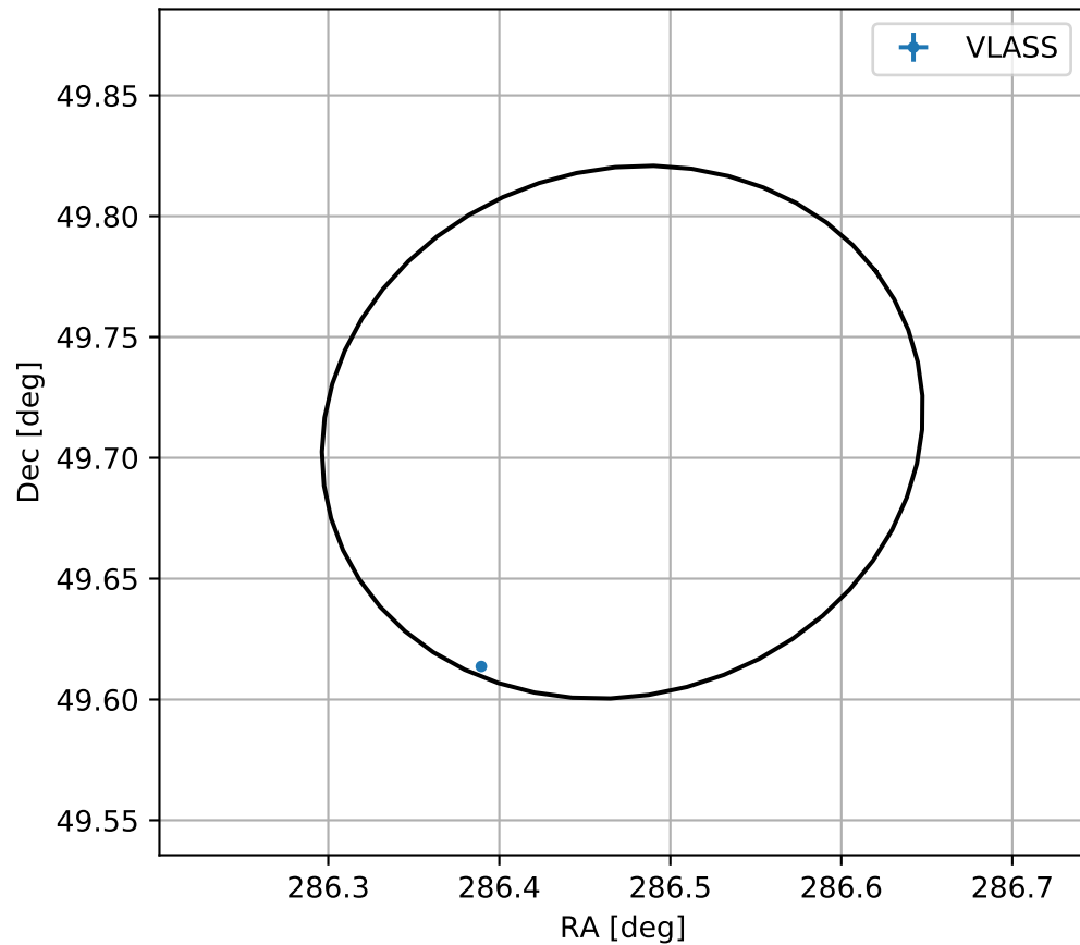
4FGL J1905.8+4942
