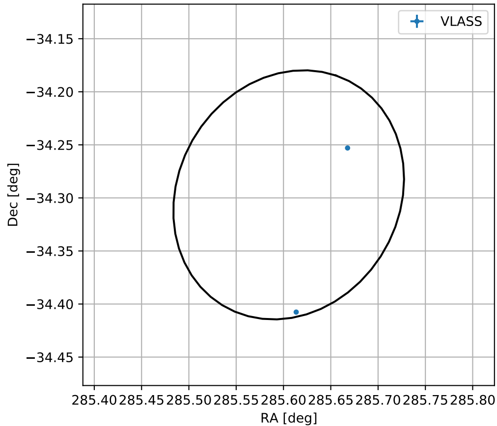
4FGL J1902.4-3417
