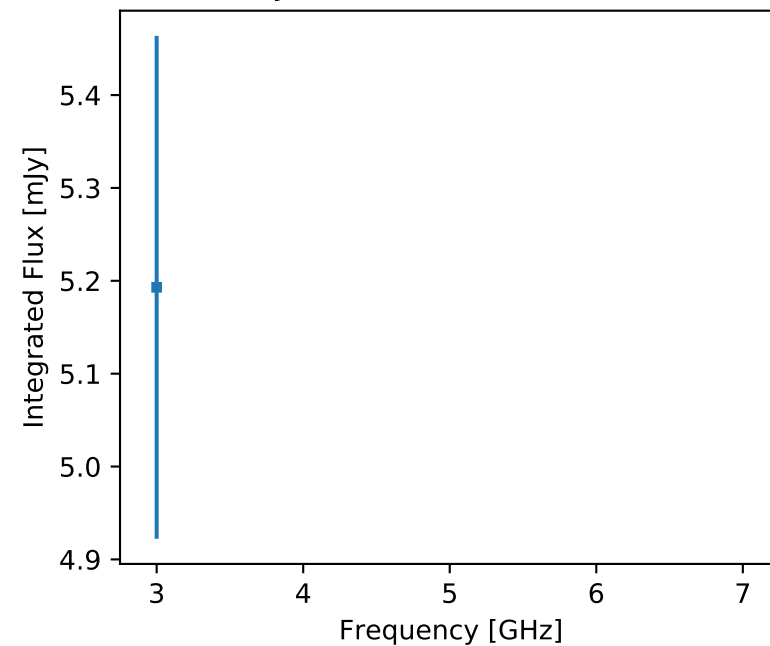
F357 J190240.25-341510.6 (unr)
