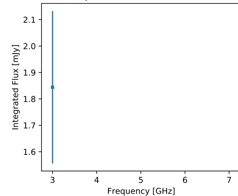
F357 J190106.64+042405.1 (unr)
