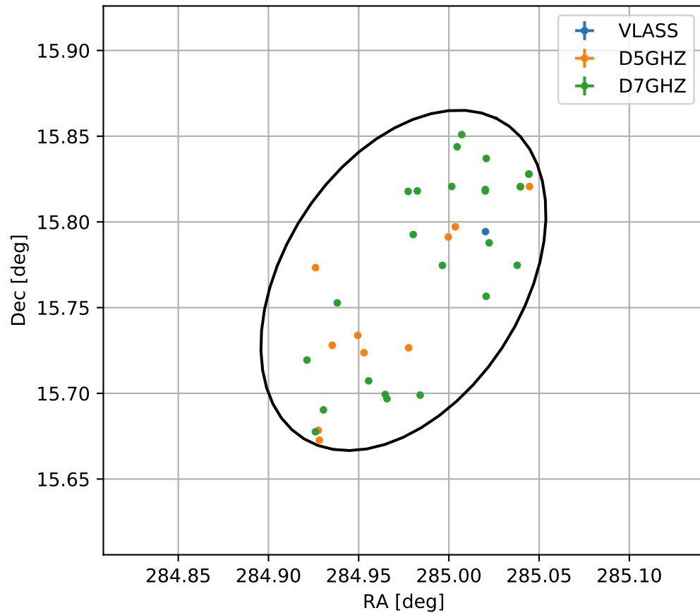
4FGL J1859.8+1545
