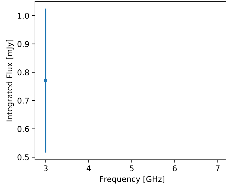
F357 J185935.96+010024.9 (unr)
